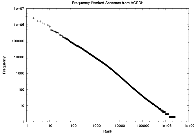
Figure 3: Distribution of frequency-ordered unique schemas in the ACSDB, with rank-order on the x-axis, and schema frequency on the y-axis. Both rank and frequency axes have a log scale.
