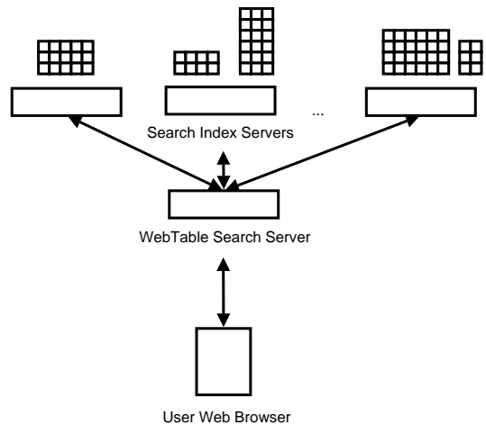
Figure 9: The WEBTABLES search system. The inverted table index is segmented by term and divided among a pool of search index servers. A single front-end search server accepts the user’s request, transmits it to all of the index servers, and returns a reply.
